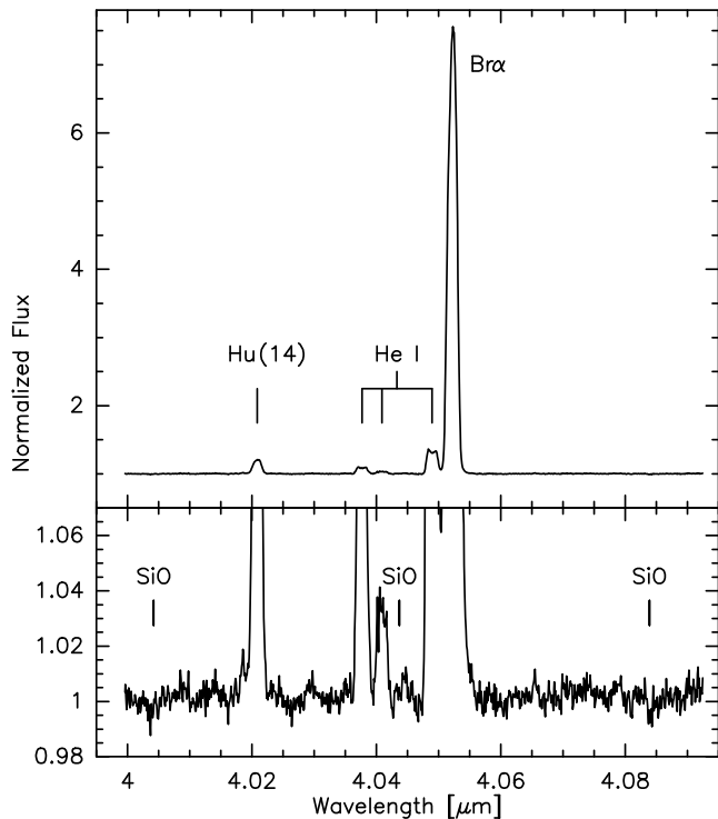
Figure 2. High-resolution L -band spectrum of MWC 349A with prominent emission lines labeled (top). The bottom panel is a zoom around the continuum, indicating the wavelengths of the SiO band heads.
