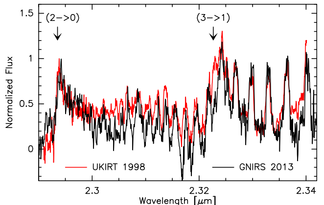
Figure 4. UKIRT spectrum taken in 1998 (red) superimposed on the GNIRS spectrum taken in 2013 (black). Marked are the positions of the ^{12}\text{CO} band heads ( 2 \rightarrow 0 ) and ( 3 \rightarrow 1 ). For easier comparison, the emission is normalized to the intensity of the first band head.
