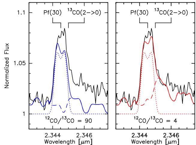
Figure 3. Model fits (color) to the observations (black) zoomed to the region around the Pf(30) line. The dashed and dotted lines represent the pure CO and pure Pfund contribution to the combined fit (solid line). The fits in the left and right panels correspond to models with ^{12}\text{CO}/^{13}\text{CO} isotope ratios of 90 and 4, respectively.
